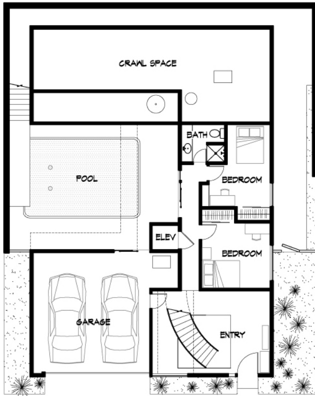
FIRST FLOOR PLAN 700 SF FLR. AREA + 420 SF GARAGE
