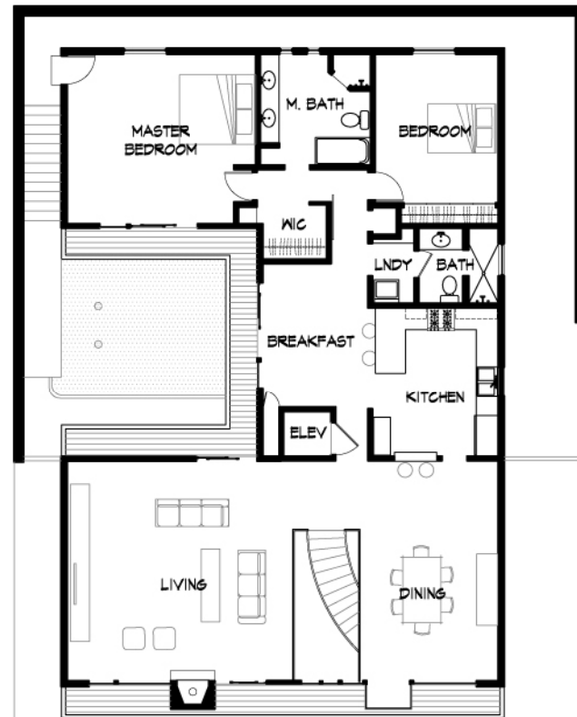
SECOND FLOOR PLAN 1800 SF FLR. AREA + 200 SF DECK
